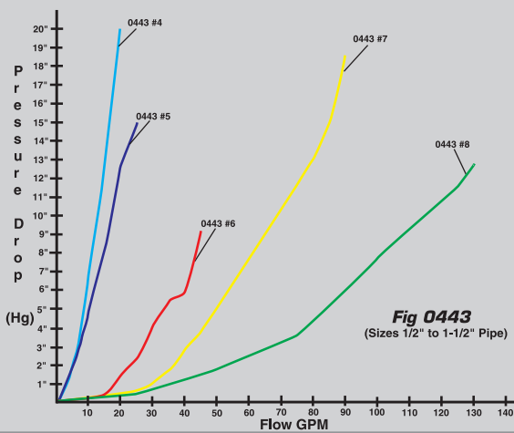
FIG. 0443 - DIFFERENTIAL PRESSURE GRAPH
